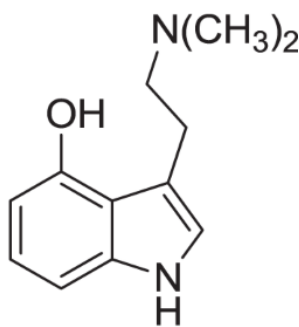
Psilocin
